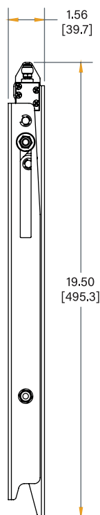
PLUMB AT 0°
